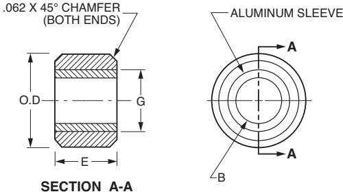
Fig. 2 (WITH CHAMFER)
