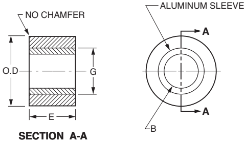
Fig. 1 (WITHOUT CHAMFER)
