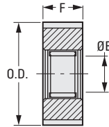
Fig. 4 Timing Pulleys 1/5 Pitch and 3 & 5 mm HTD®
